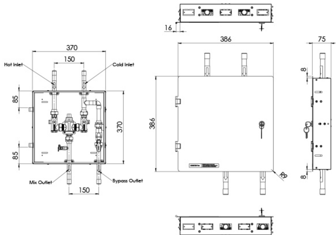
42455 Home TMV Box with: • Stainless Steel hinged door • Key locks • Pipes at both ends - Bypass
