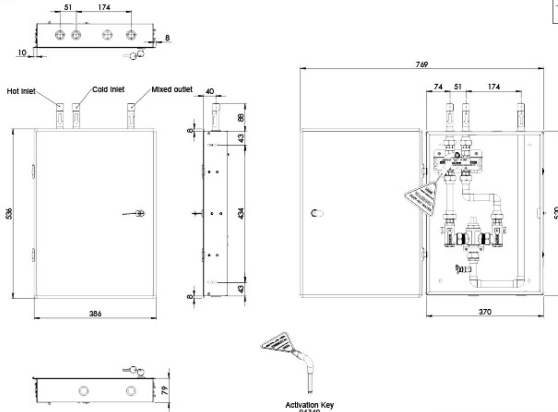
ILTDO & TMV In Wall Box 42557
