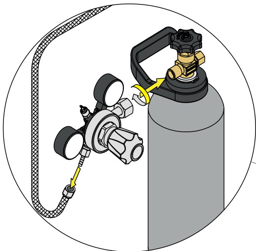
CO 2 regulator
