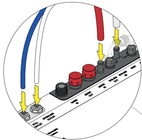
Tap connections
