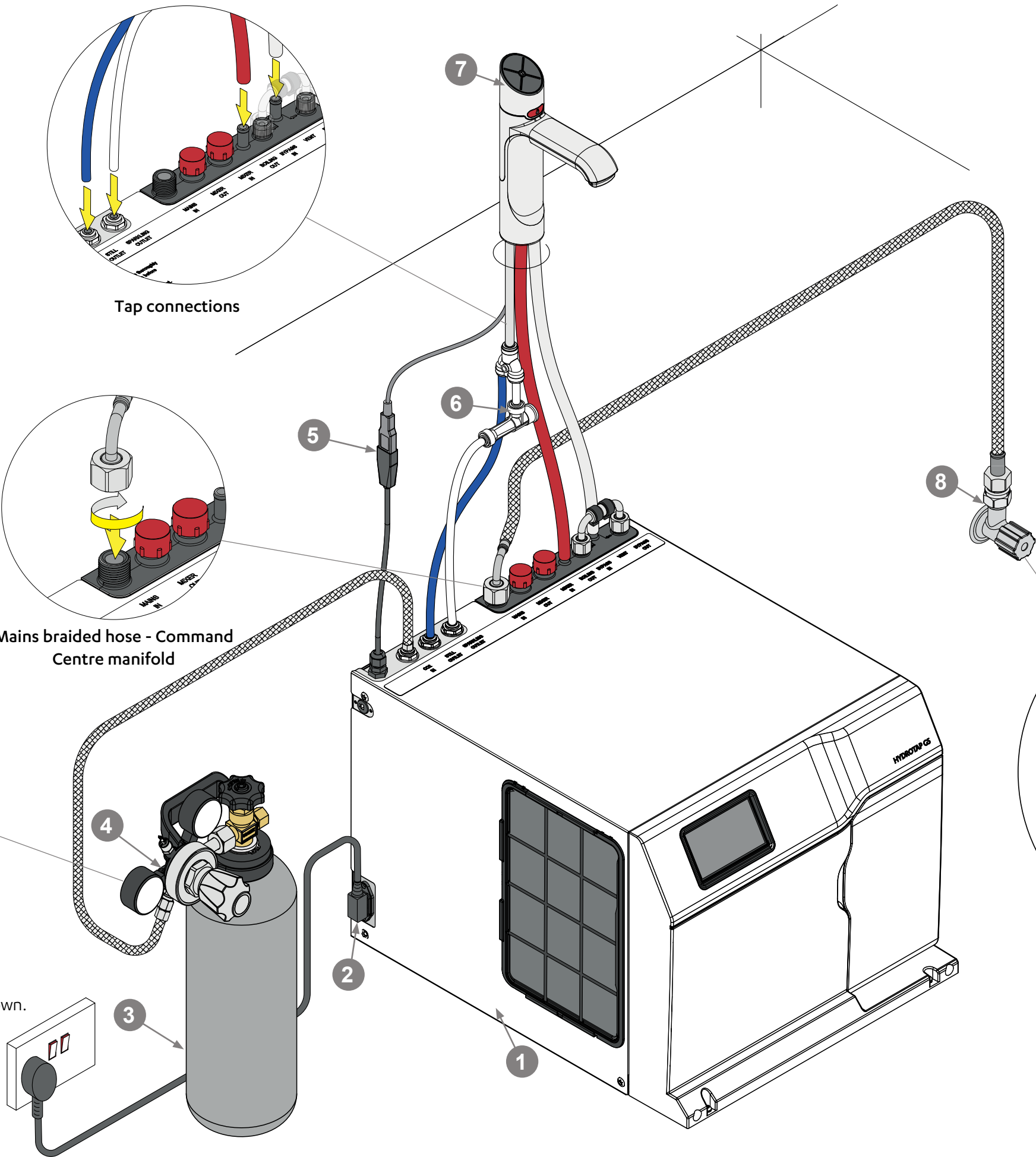
Mains braided hose - Command Centre Water supply connection
