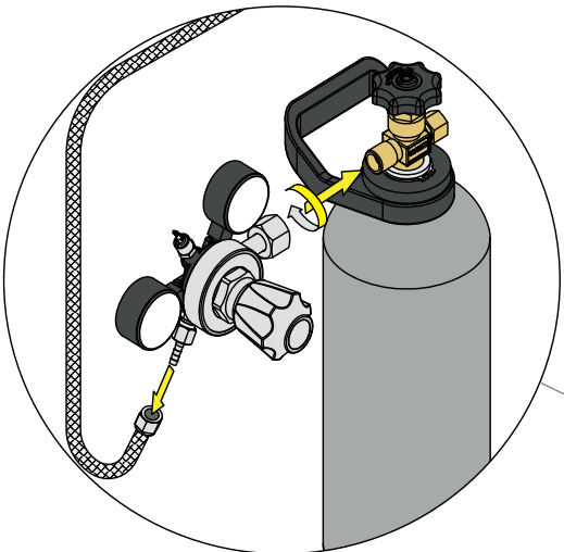
CO 2 regulator
