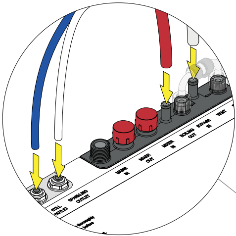
Tap connections
