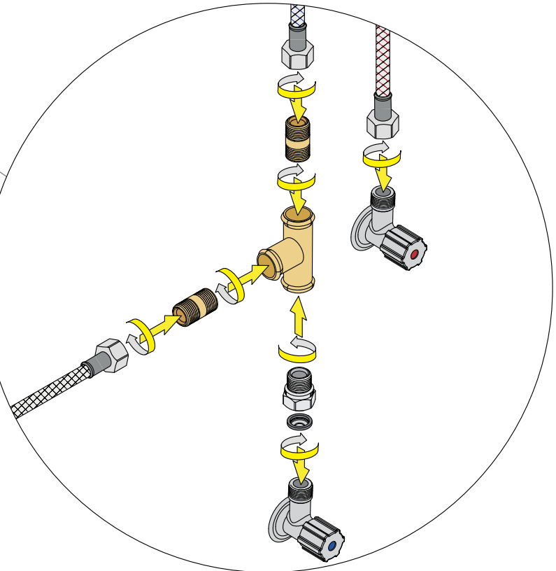
Mains braided hose - Command Centre Water supply connection
