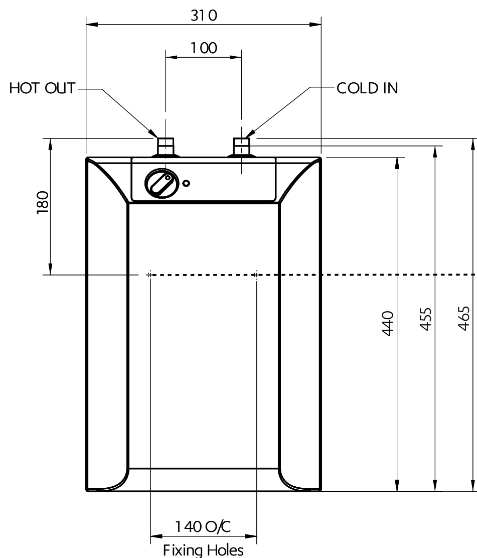
FRONT VIEW SCALE 1 : 5
