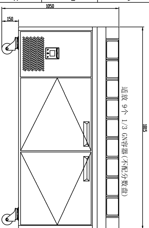
ELEVATION ???
