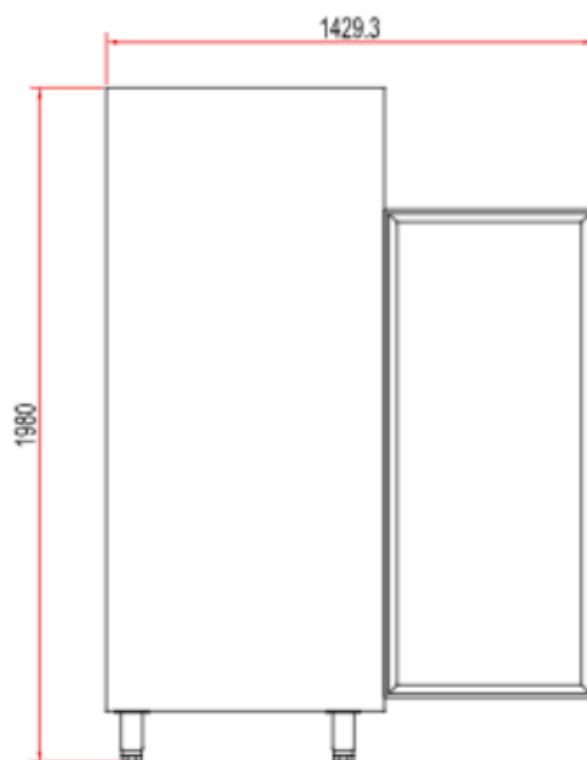
SIDE VIEW 左侧视图
