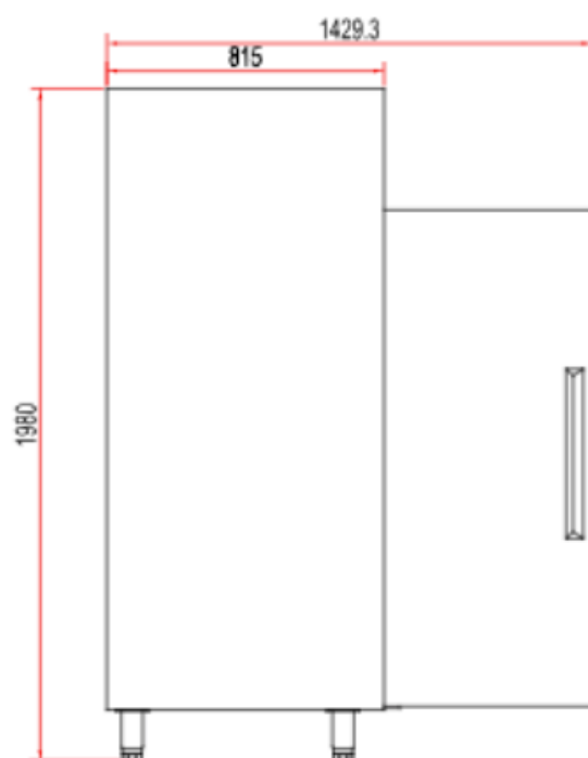
SIDE VIEW 左侧视图
