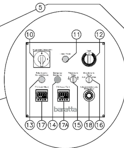
CONTROL PANEL
