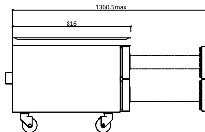
DRAWER(except GAN PAN)
