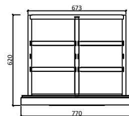
DRAWER(except GAN PAN)
