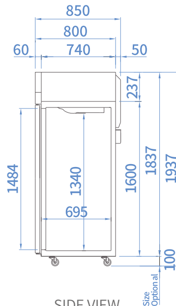
SIDE VIEW (Full Door)
